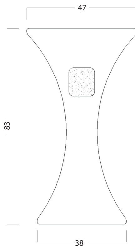
LATERAL VIEW
