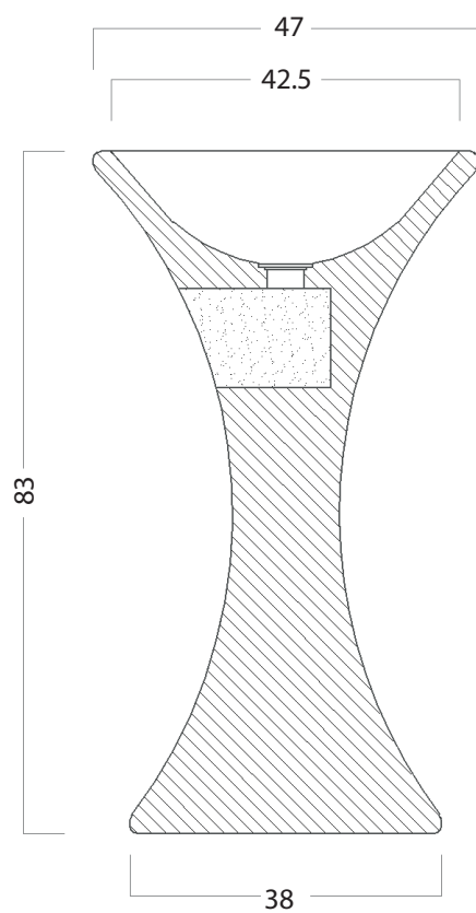
SECTION
