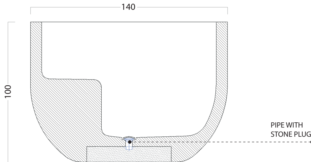
SECTION
